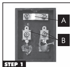
Connect Terminal Box
